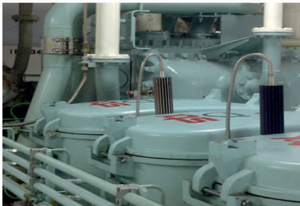
HTT-04CA sensors mounted on Thompson adaptors on a 4-stroke diesel engine
